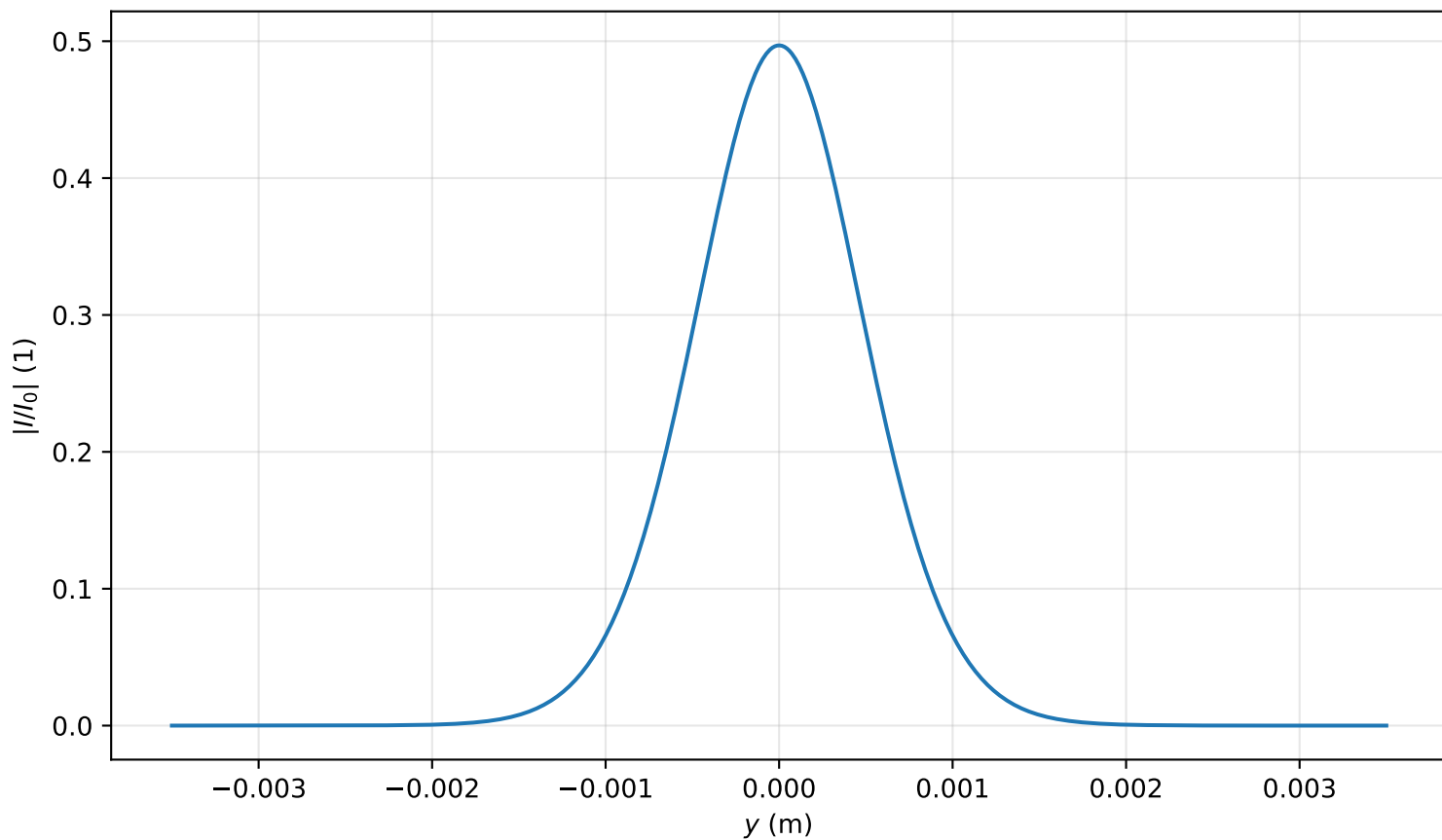
Intensity profile I(x=0, y, z=2.627)/I_0 , P_{in}=0.3P_{cr} , artificial time
